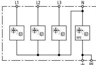
Basic circuit diagram DSH TT 255
